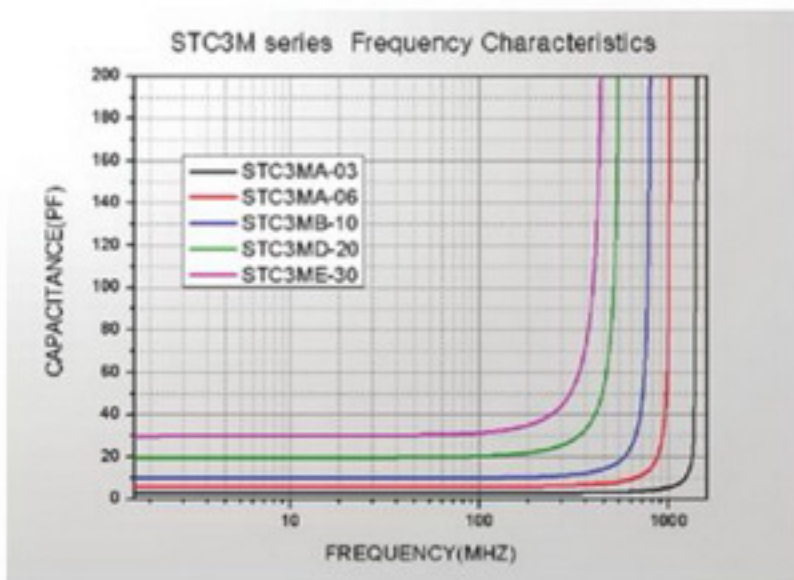
Capacitance vs Frequency Curve 容量与频率特性曲线
