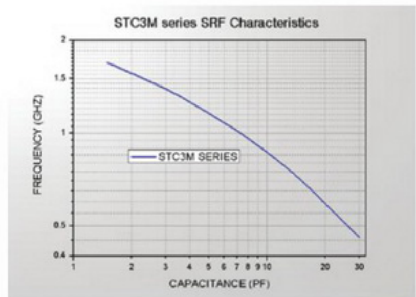
Self-Resonant Frequency Curve 自谐振频率曲线
