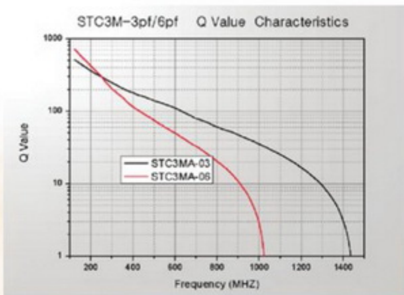
Q Values vs Frequency Curve Q值与频率特性曲线
