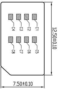
REFERENCE SIM CARD PLUG SCALE 1:2
