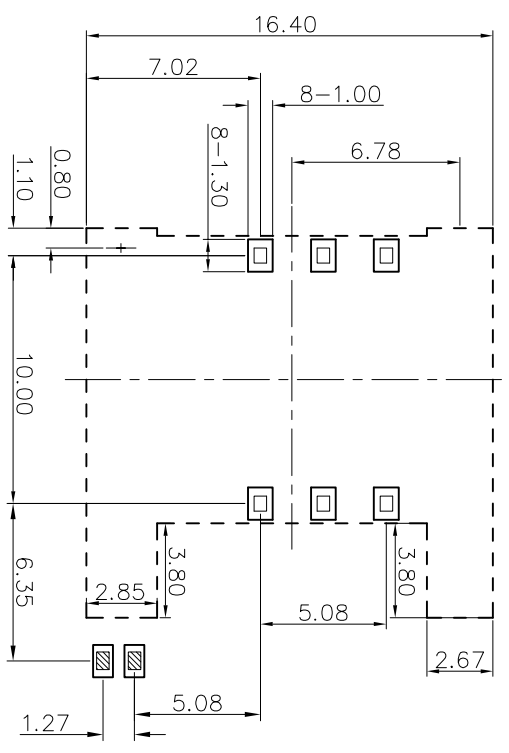
REFERENCE PC BOARD LAYOUT
